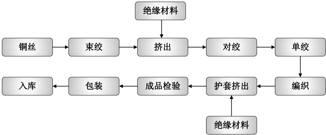
(8) 充电线缆
